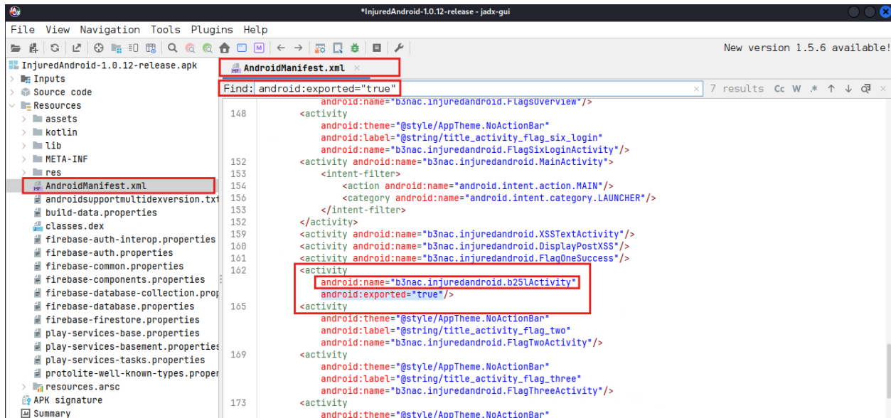
Figure 1: Analyzing AndroidManifest.xml for Exported Activities by Searching for the String (android:exported="true") and Found an Activity of Class "b3nac.injuredandroid.b25lActivity"
